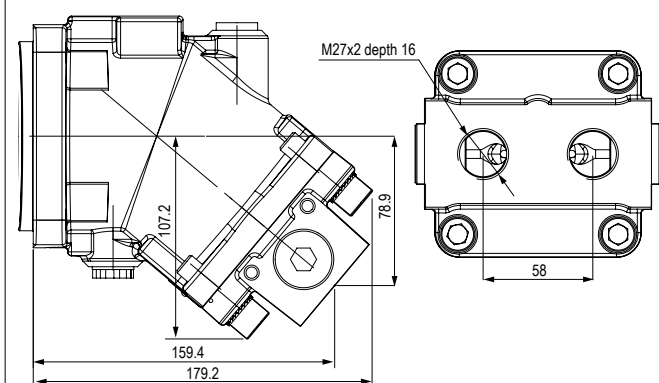
P0 Rear threaded ports A and B
