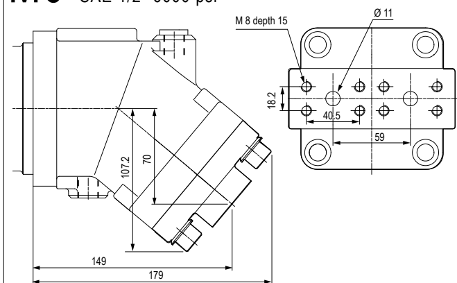
M0 Rear flange ports A and B SAE 1/2" 6000 psi
