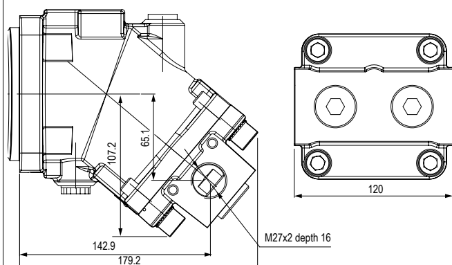
Q0 Side threaded ports
